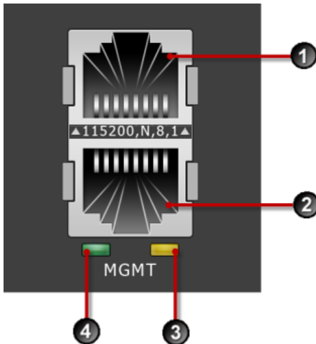
FIGURE 4. Console and management ports
