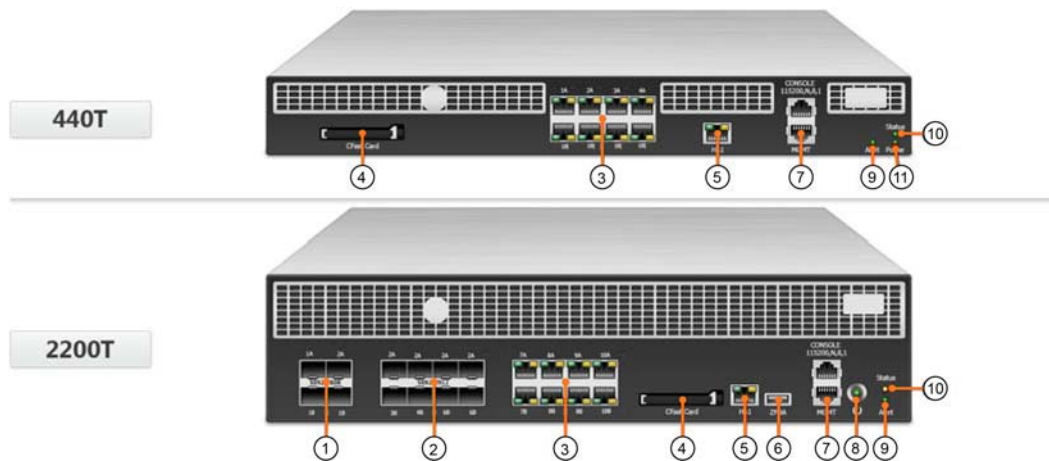
Figure 1. TippingPoint TPS 440T and 2200T security devices – front panel
