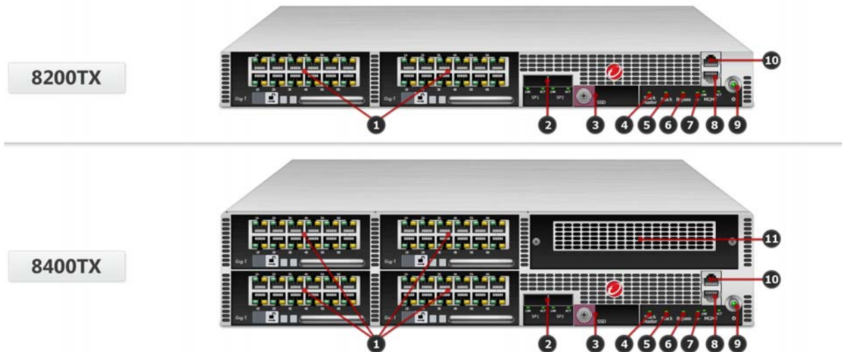
Figure 1. TippingPoint TPS 8200TX and 8400TX security devices – front panel
