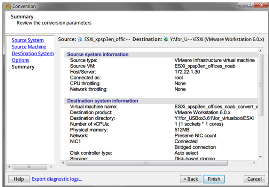
FIGURE 3-19. Conversion > Summary
