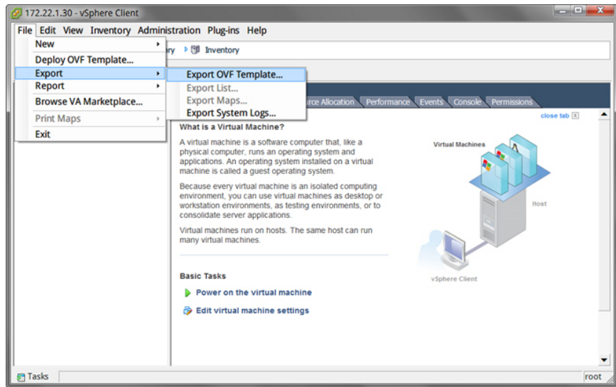
FIGURE 3-14. OVF Template
