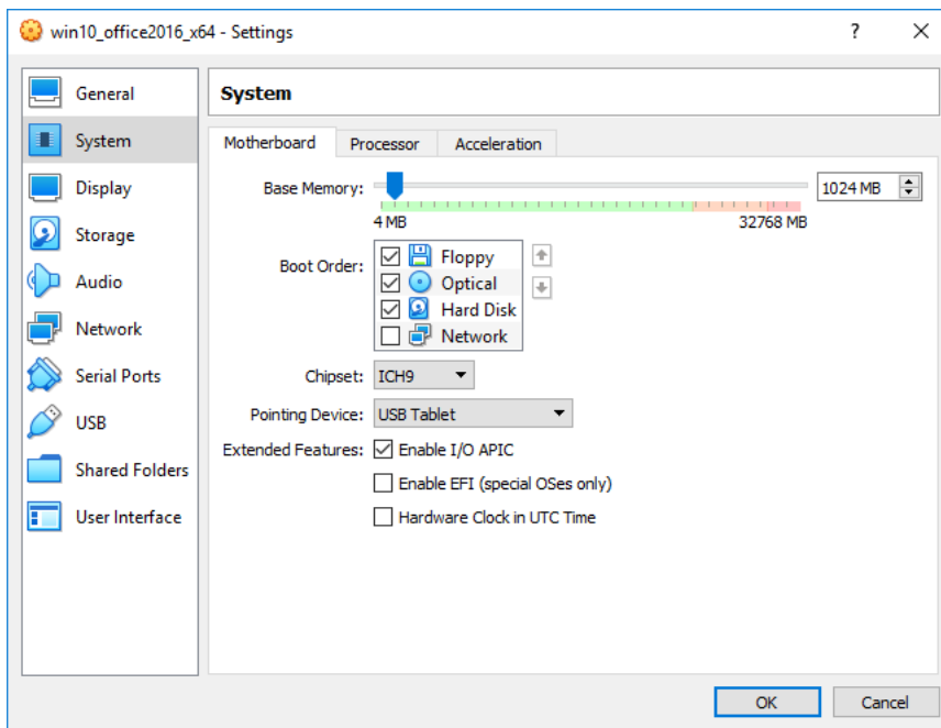
FIGURE 3-29. System Screen
