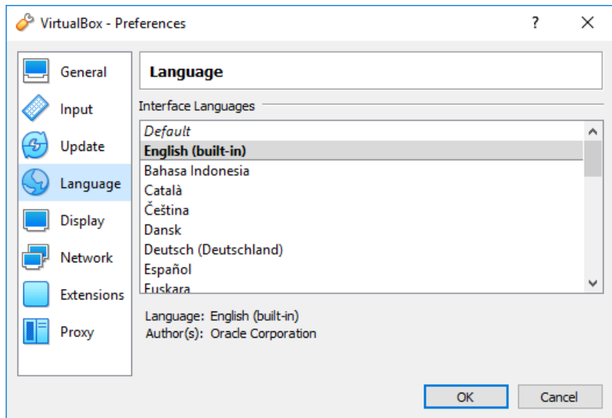
FIGURE 2-3. Language Settings
