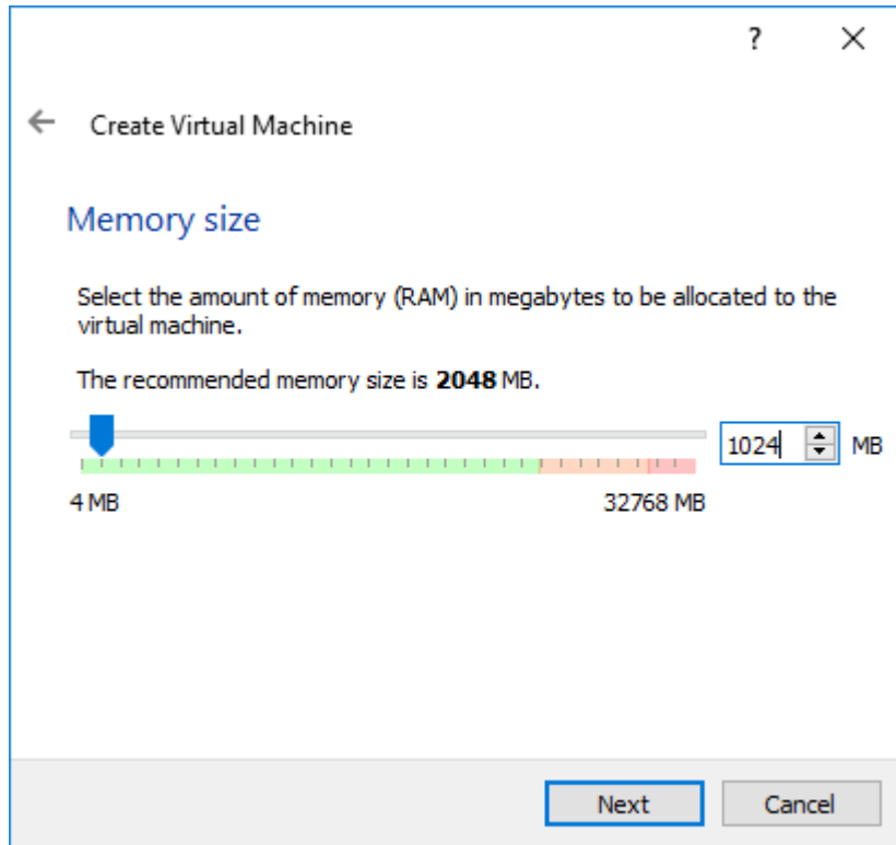
FIGURE 3-24. Memory Size
