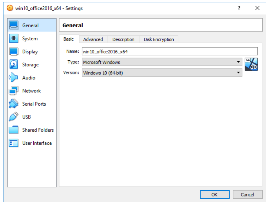
FIGURE 3-28. VirtualBox Settings
