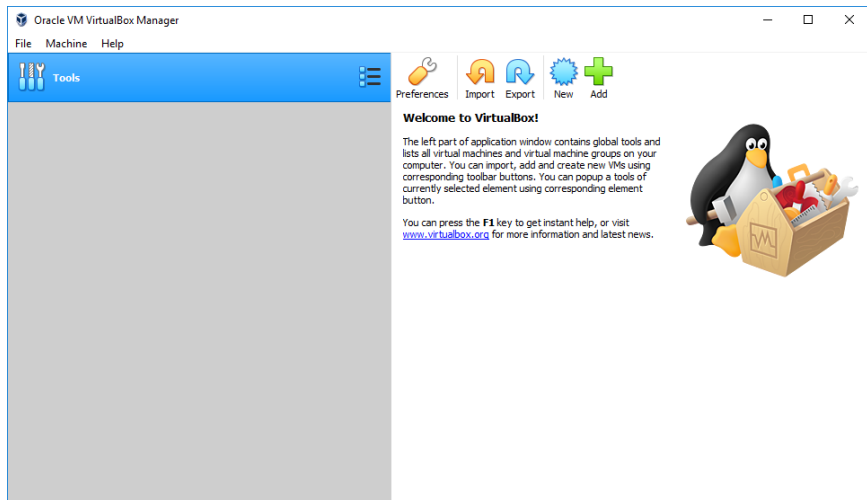
FIGURE 3-22. VirtualBox Manager
