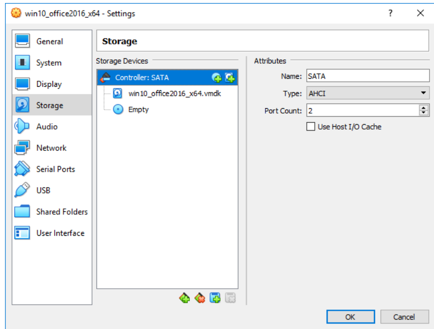
FIGURE 2-14. Storage Screen
