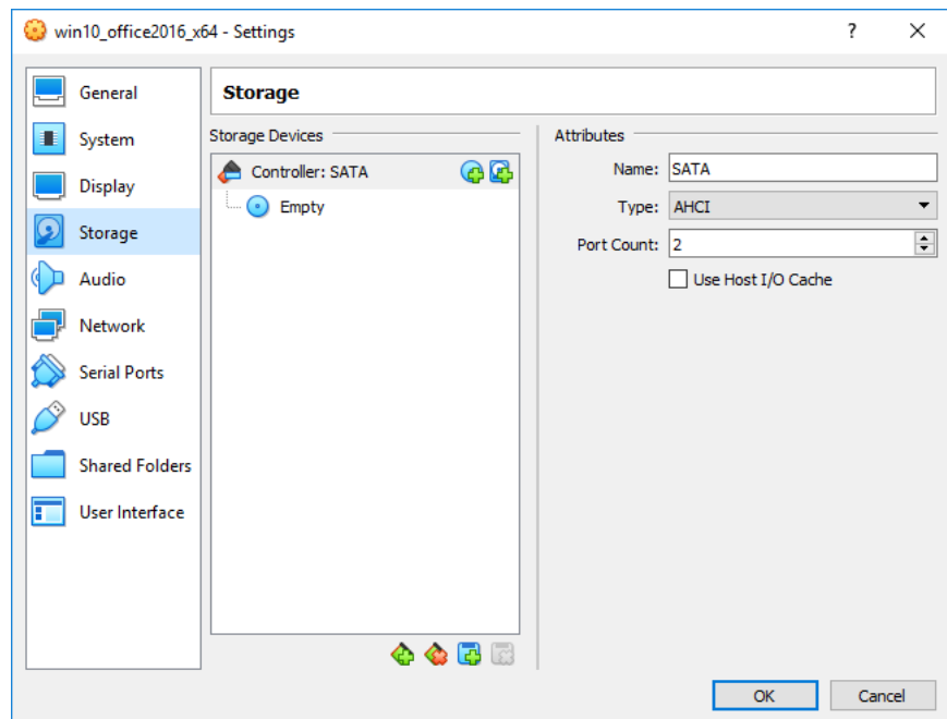
FIGURE 3-30. Storage Screen
