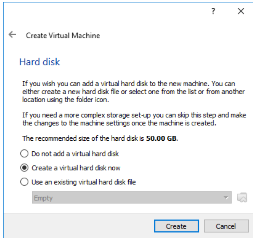
FIGURE 2-7. Hard Disk
