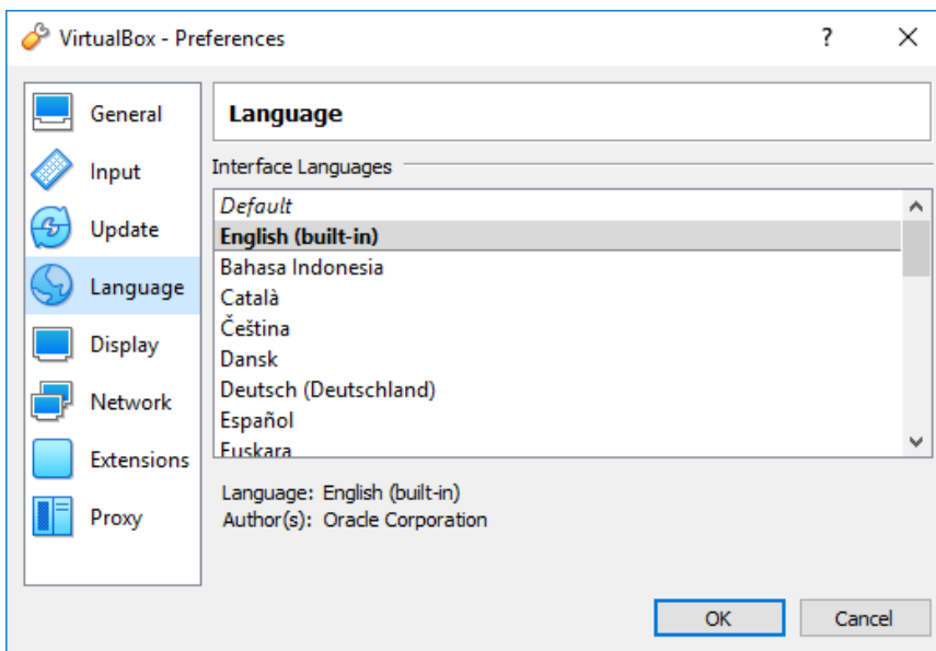
FIGURE 3-21. Language Settings
