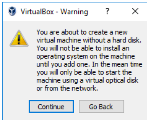
FIGURE 3-26. Warning
