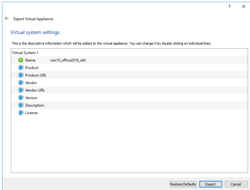
FIGURE 2-29. Appliance settings
