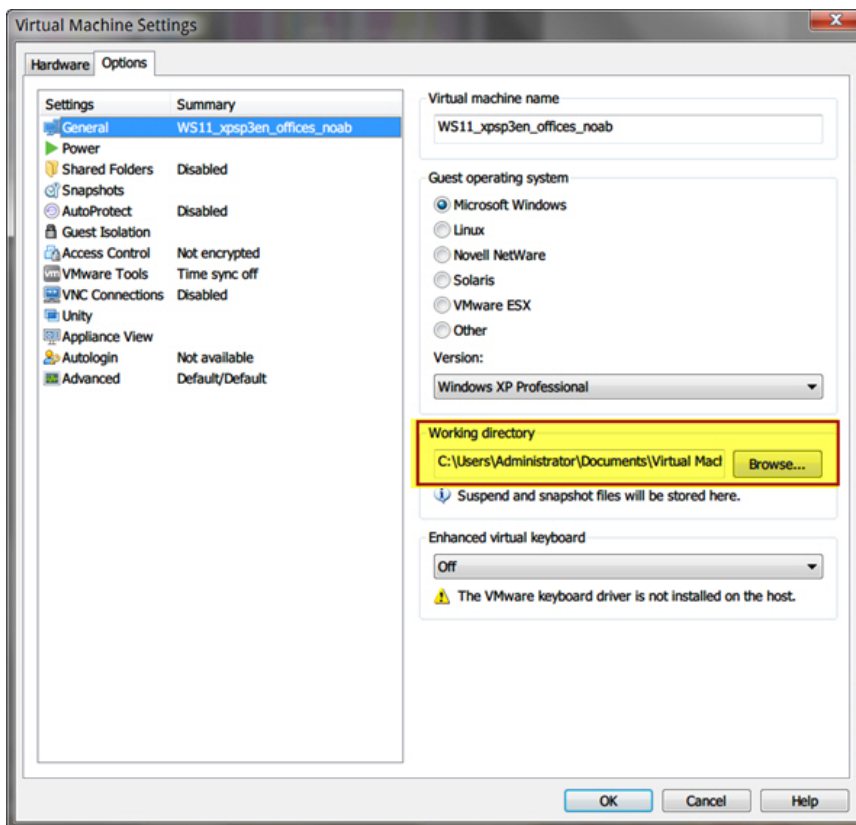
FIGURE 3-11. Working Directory
