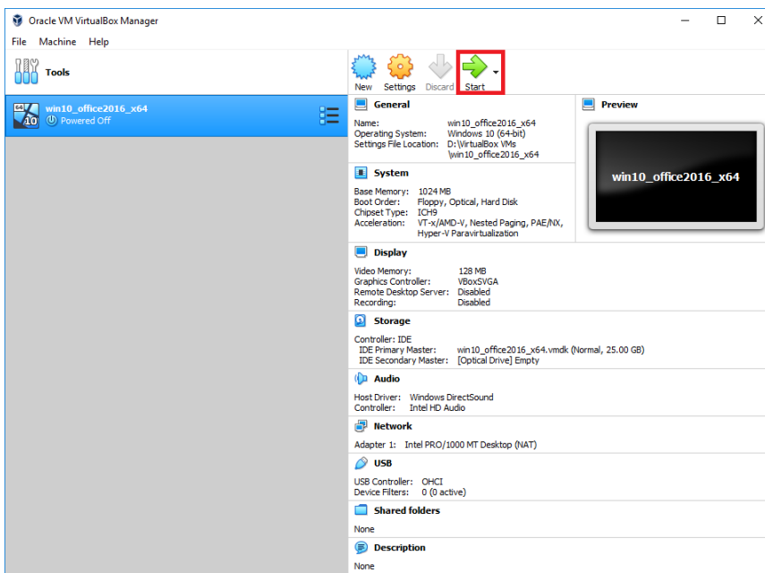
FIGURE 3-37. VirtualBox Manager
