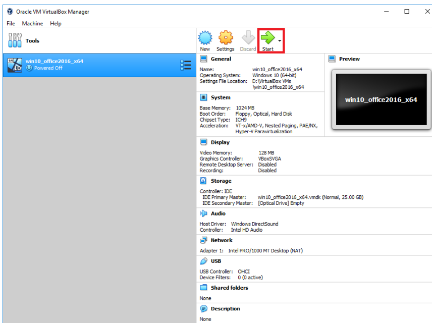
FIGURE 2-21. VirtualBox Manager
