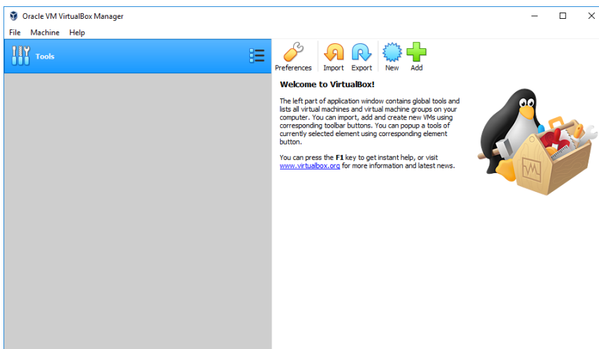
FIGURE 2-4. VirtualBox Manager
