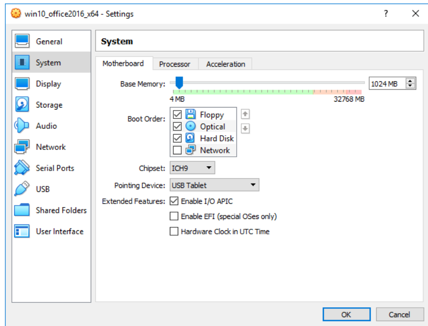
FIGURE 2-13. System Screen
