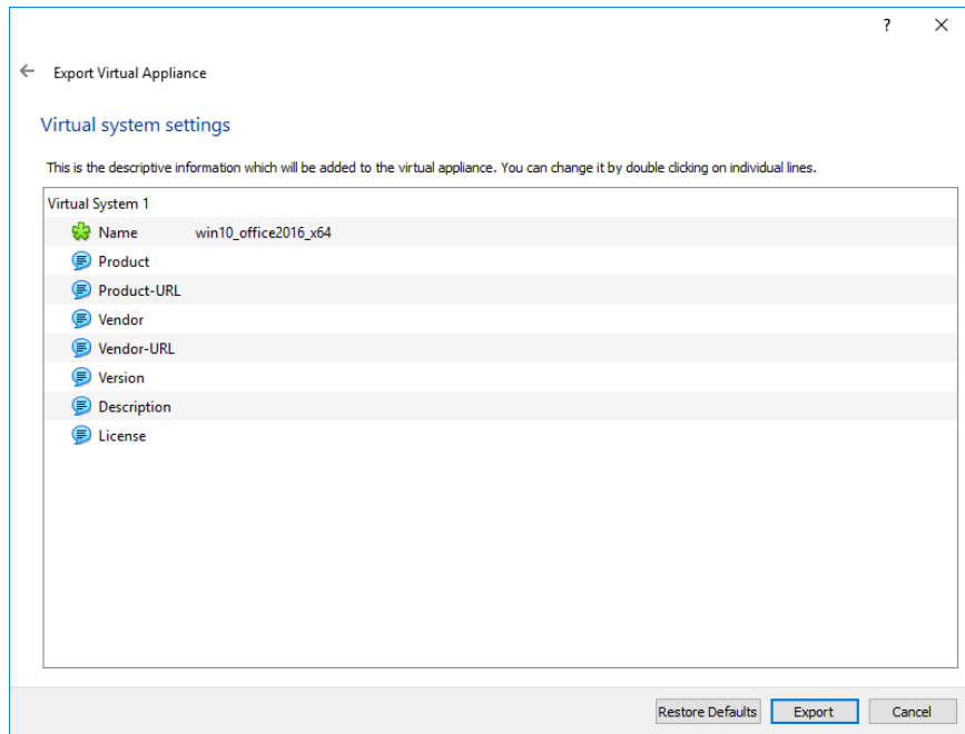
FIGURE 3-43. Appliance settings
