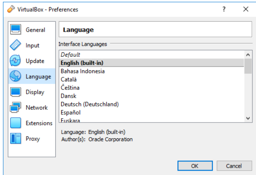
FIGURE 3-20. Language Settings
