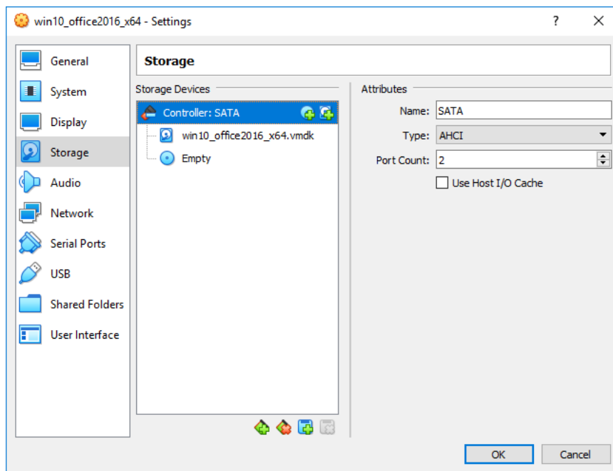
FIGURE 2-13. Storage Screen
