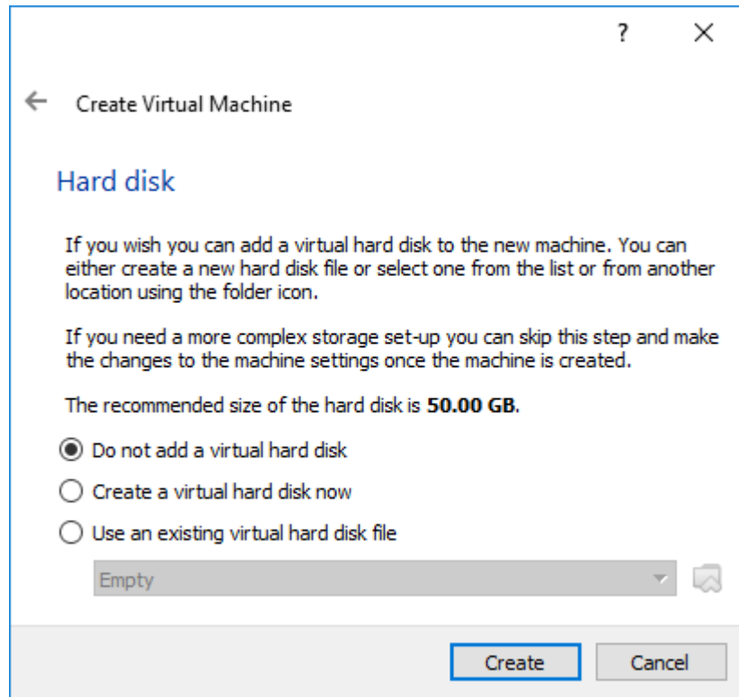
FIGURE 3-24. Hard Disk
