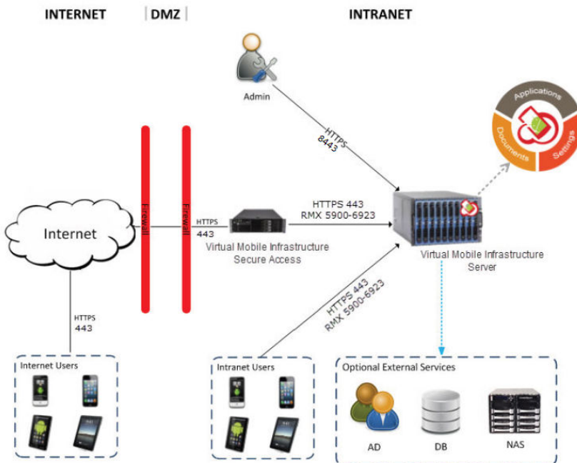
FIGURE A-1. Network Ports in Virtual Mobile Infrastructure Architecture
