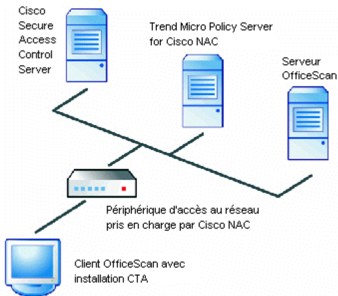
FIGURE 15-1. Architecture Cisco NAC de base
