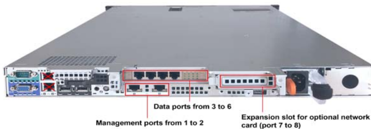
FIGURE 2-6. Standard six-port configuration
