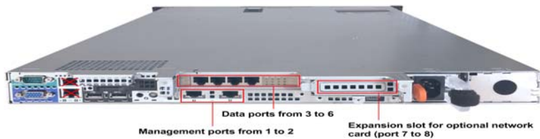
FIGURE 2-7. Standard six-port configuration
