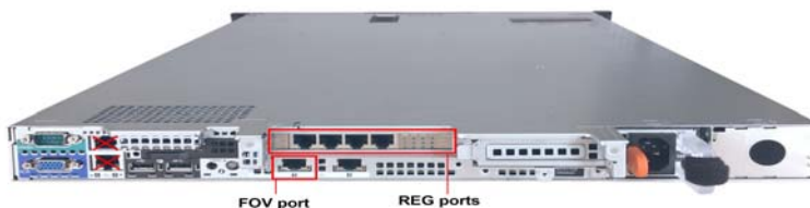
FIGURE 3-12. Interface allocation for a port grouping with failover deployment
