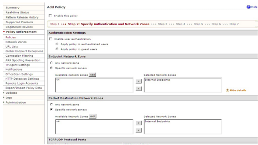
FIGURE 4-13. Specifying the network zone
