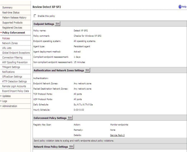
FIGURE 4-16. Reviewing the policy and enabling it
