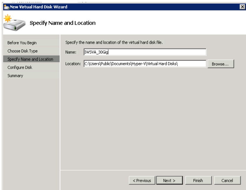
FIGURE F-16. Specify Hard Drive Name and Location
