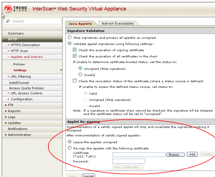
FIGURE 4-4. Re-import the Applet Re-signing Certificate
