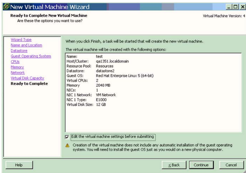
FIGURE E-11. Ready to Complete
