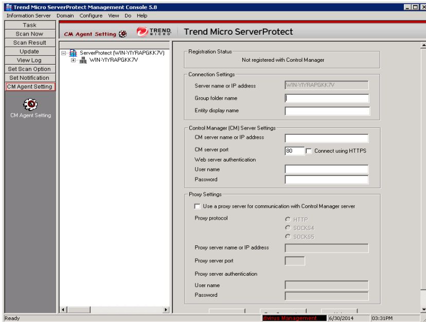
FIGURE 3-71. CM Agent Setting screen
