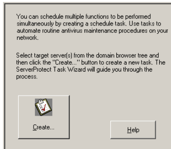
FIGURE 3-34. Configuration Area
