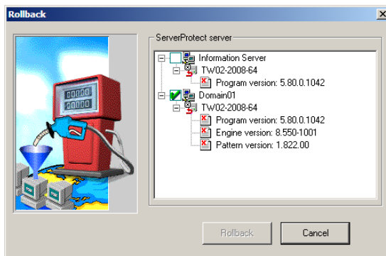
FIGURE 3-46. Rollback window
