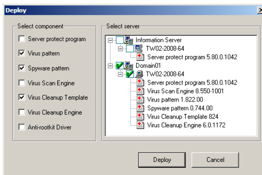
FIGURE 3-43. Deploy window
