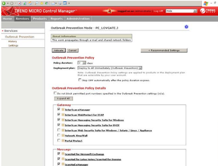
FIGURE 5-74. Services screen
