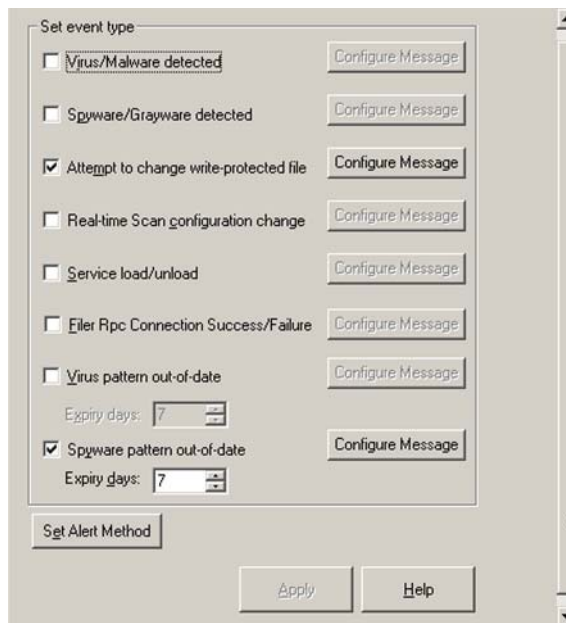
FIGURE 3-32. ServerProtect Standard Alert Configuration Window
