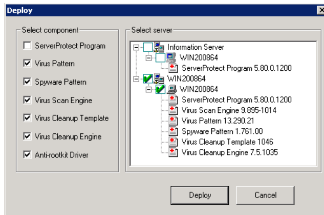
FIGURE 4-2. The Deploy Window
