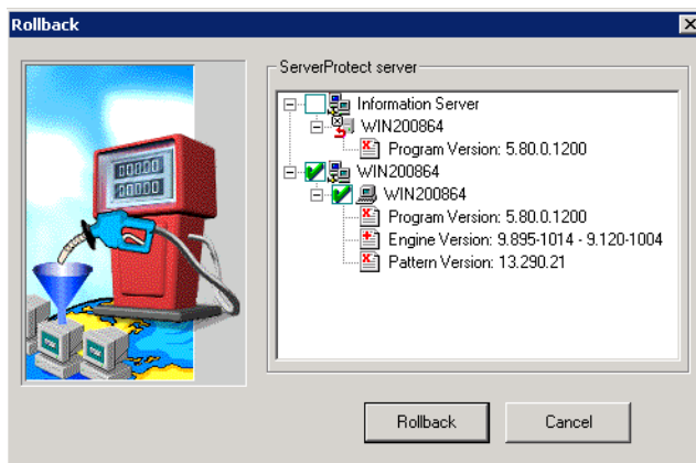
FIGURE 3-21. Rollback dialog
