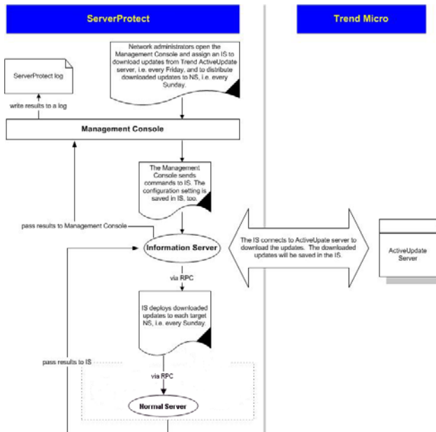
FIGURE 3-13. How Updates Work
