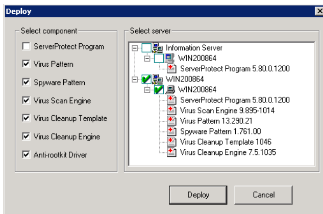
FIGURE 3-18. Deploy dialog
