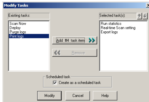
FIGURE 3-30. Modify Tasks dialog
