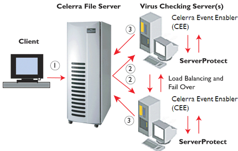
FIGURE 1-2. ServerProtect for EMC Celerra Architecture
