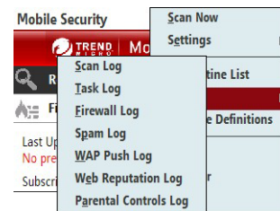
Figure 9-11. Event logs
