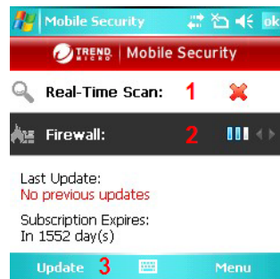
Figure 3-1. Main screen
